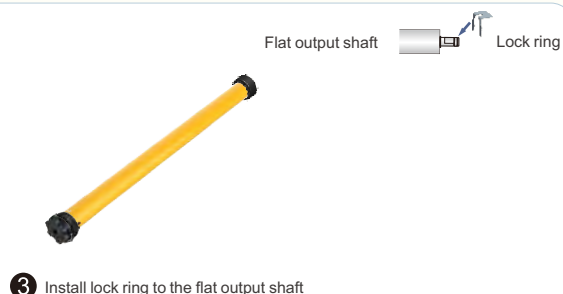
③ Install lock ring to the flat output shaft
