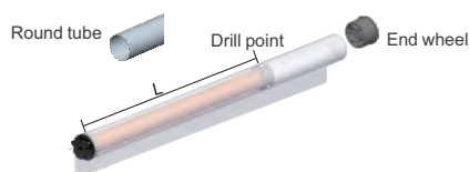
Marked drill position on the tube, and insert end wheel
